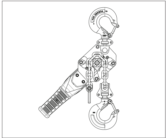
Chain Installation Single Reeved (0.75 – 3 Tonne)
