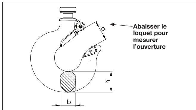
Figure 5 - Inspection du crochet
