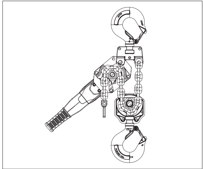
Chain installation Double Reeved (6 Tonne)
