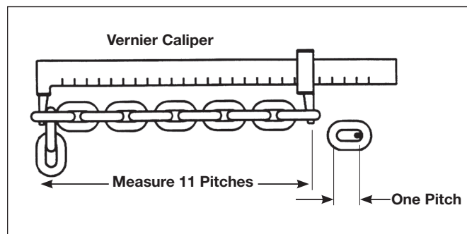
Figure 7 - Chain Inspection
