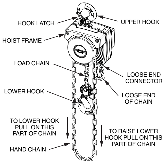
Figure 2 – Main Parts of Coffing® LHH-NC Hoist
