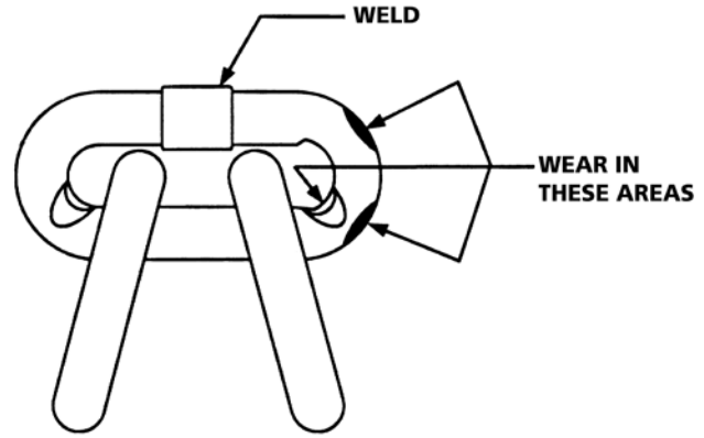
Figure 4 - Chain Inspection
