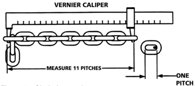
Figure 5 - Chain Inspection
