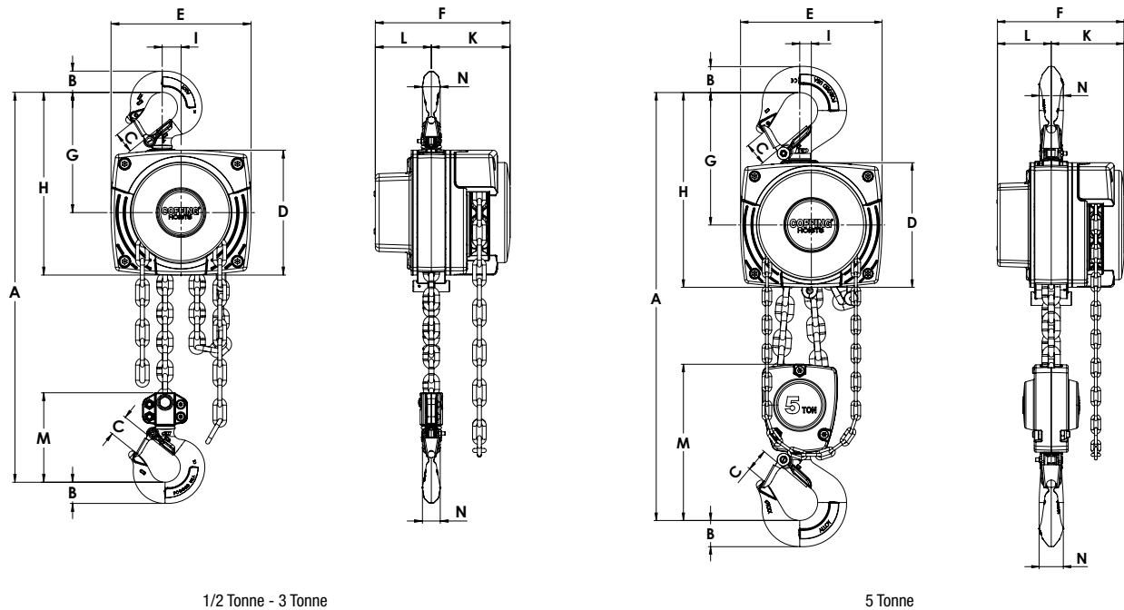
Figure 1 – Specifications & Dimensions
