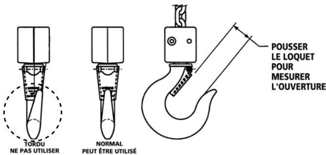
Figure 3 – Inspection du crochet
