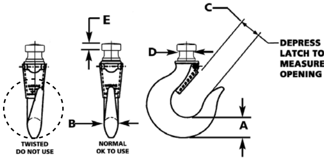
Figure 3 – Hook Inspection
